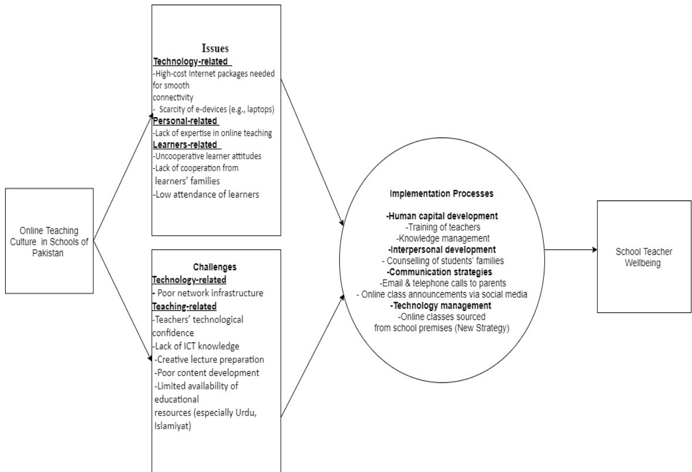
Figure 3: Conceptual Framework
